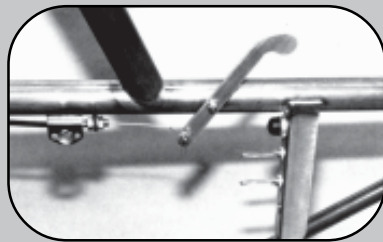
Parachute Release Handle & Cable, Switch Panel
