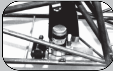
Fuel Cell, Fuel Pump / Filler Mounts
